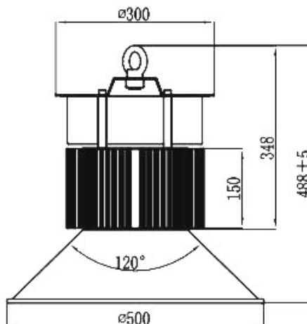
400w DIMENSIONS
